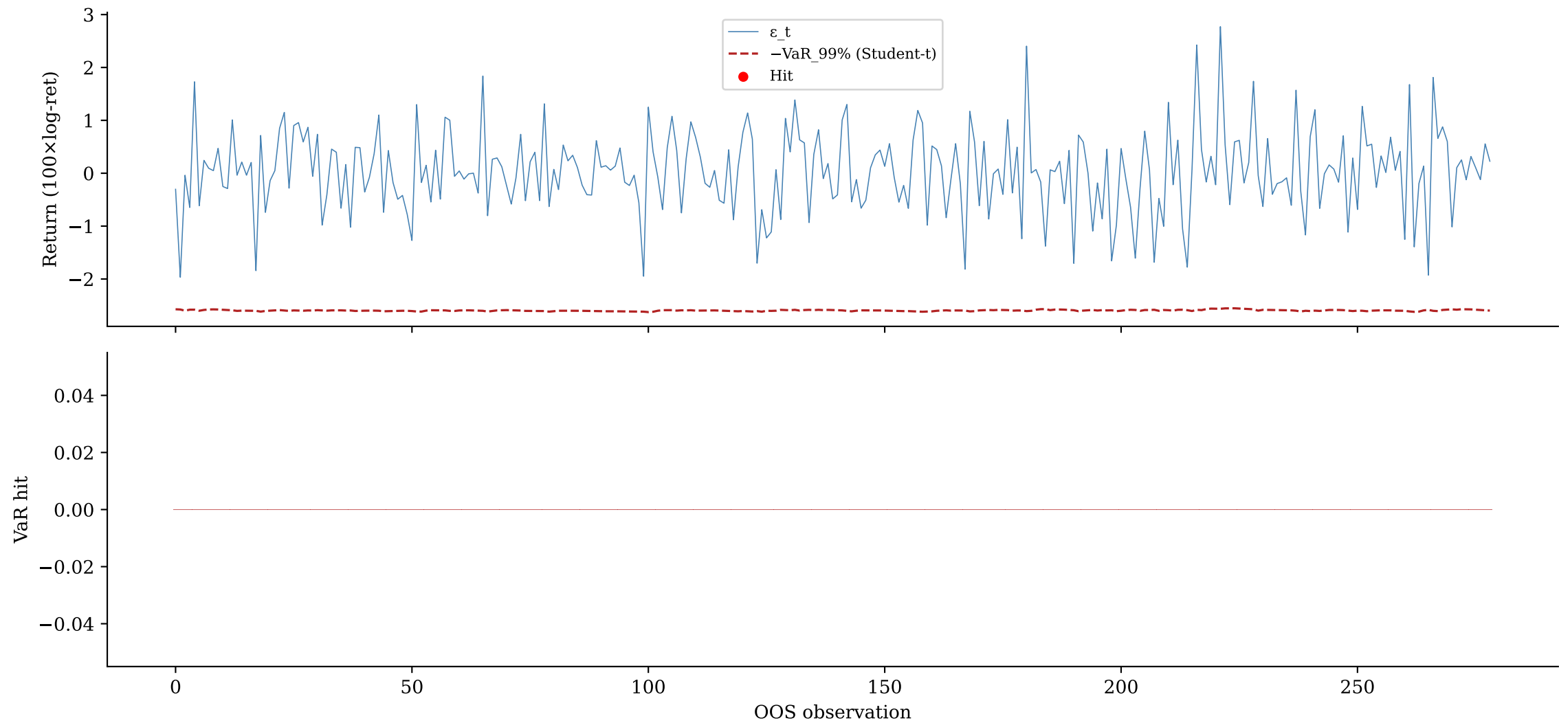
LSTM-SSE-t-Student — DJIA VaR 99% Hit Sequence
